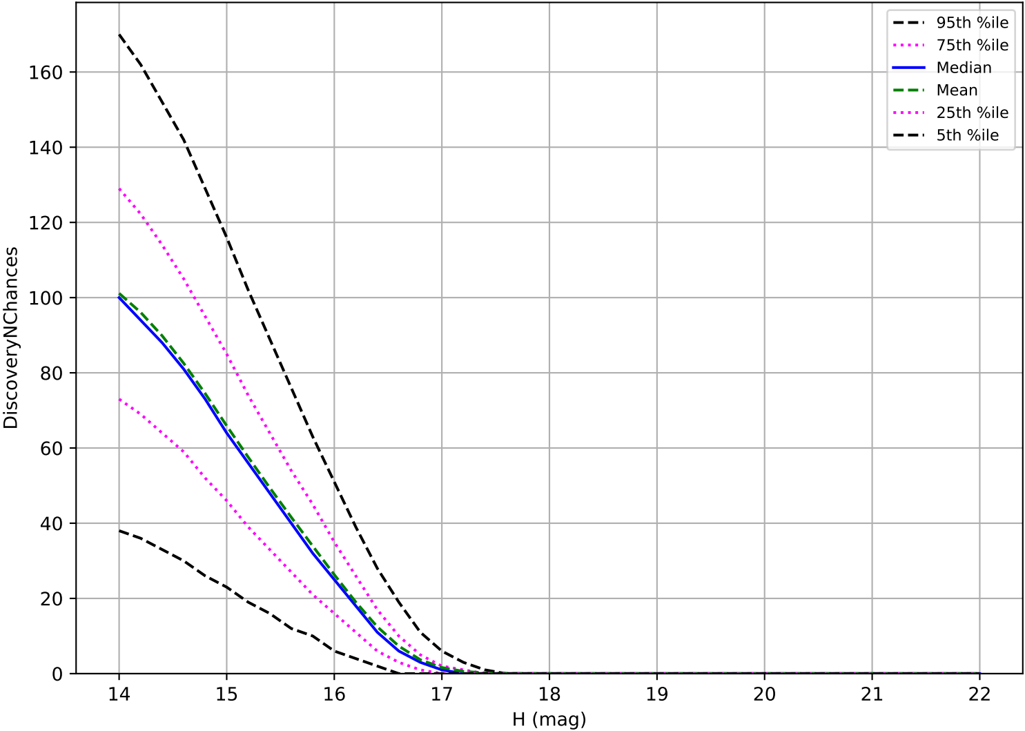
too_elab_r16_d3_giz_v3.4_10yrs: Trojan 3 pairs in 15 nights detection loss
