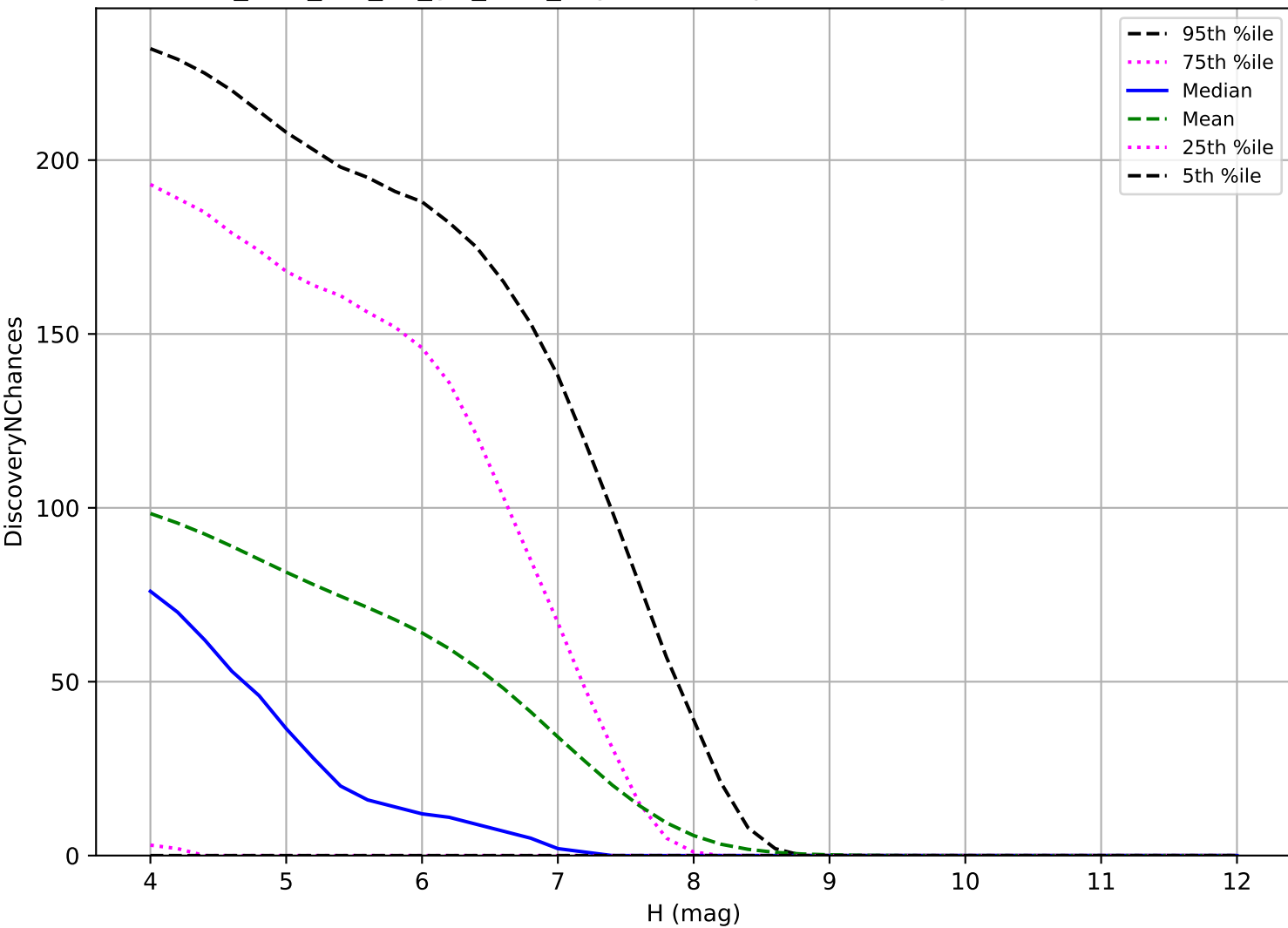
too_elab_r16_d3_giz_v3.4_10yrs: TNO 3 pairs in 15 nights detection loss
