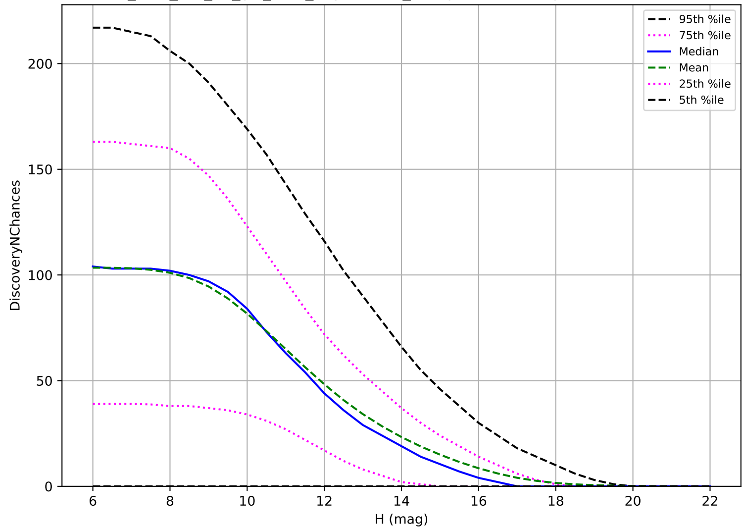
too_elab_r16_d3_giz_v3.4_10yrs: OCC_r5 3 pairs in 15 nights detection loss
