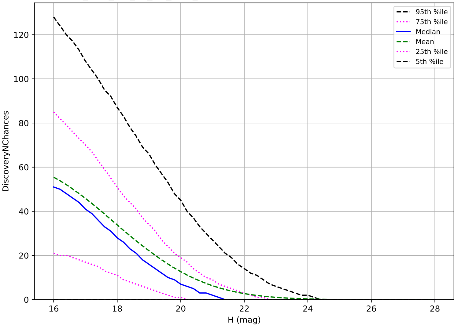
too_elab_r16_d3_giz_v3.4_10yrs: NEO 3 pairs in 15 nights detection loss
