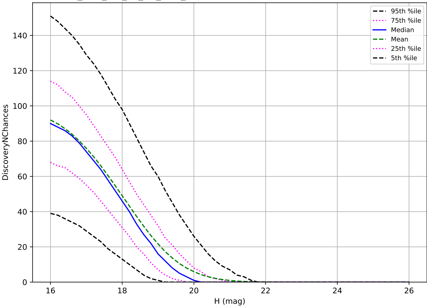
too_elab_r16_d3_giz_v3.4_10yrs: MBA 3 pairs in 15 nights detection loss
