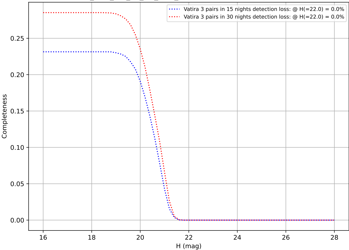
too_elab_r16_d3_giz_v3.4_10yrs: DifferentialCompleteness
