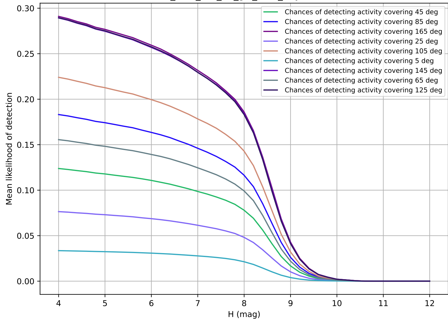
too_elab_r16_d3_giz_v3.4_10yrs TNO
