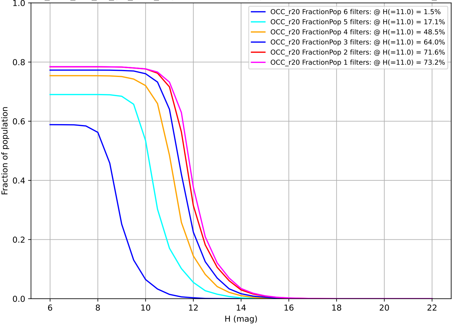
too_elab_r16_d3_giz_v3.4_10yrs: Fraction of population with colors in X filters OCC_r20
