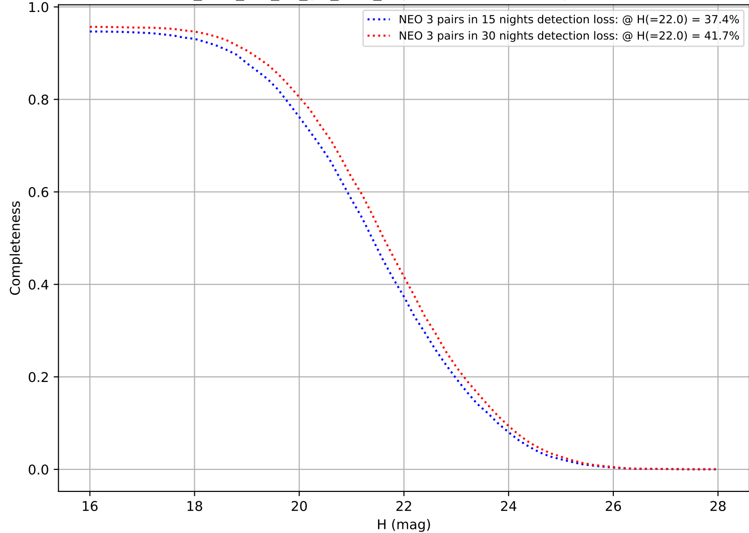
too_elab_r16_d3_giz_v3.4_10yrs: DifferentialCompleteness
