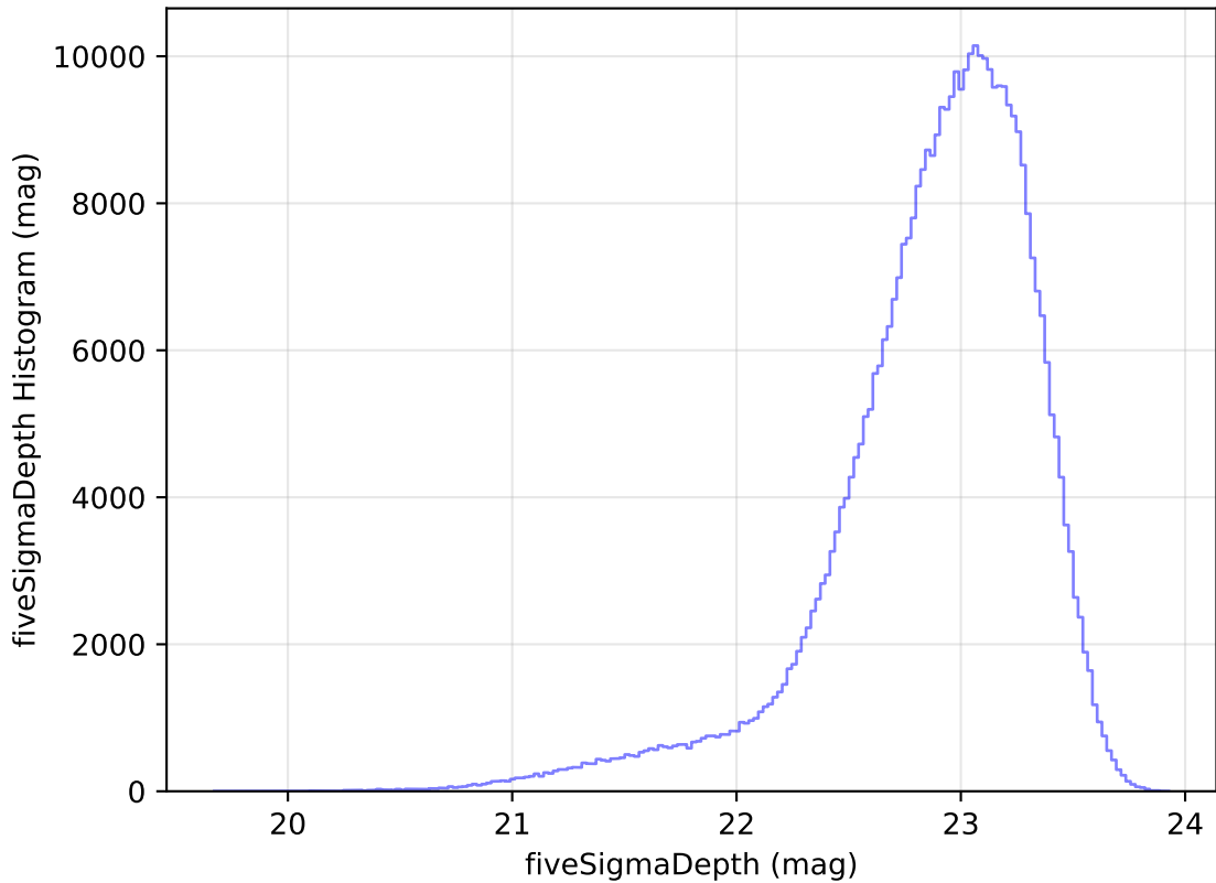
too_elab_r16_d3_giz_v3.4_10yrs z: fiveSigmaDepth Histogram
