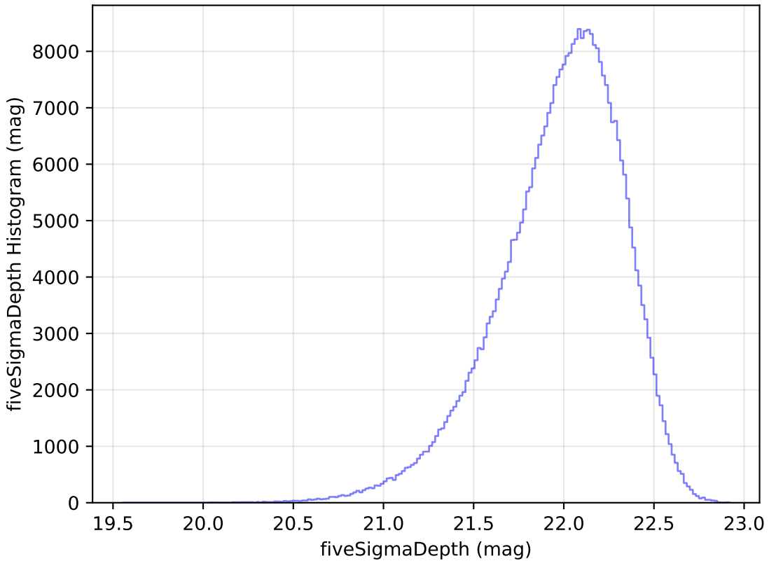
too_elab_r16_d3_giz_v3.4_10yrs y: fiveSigmaDepth Histogram
