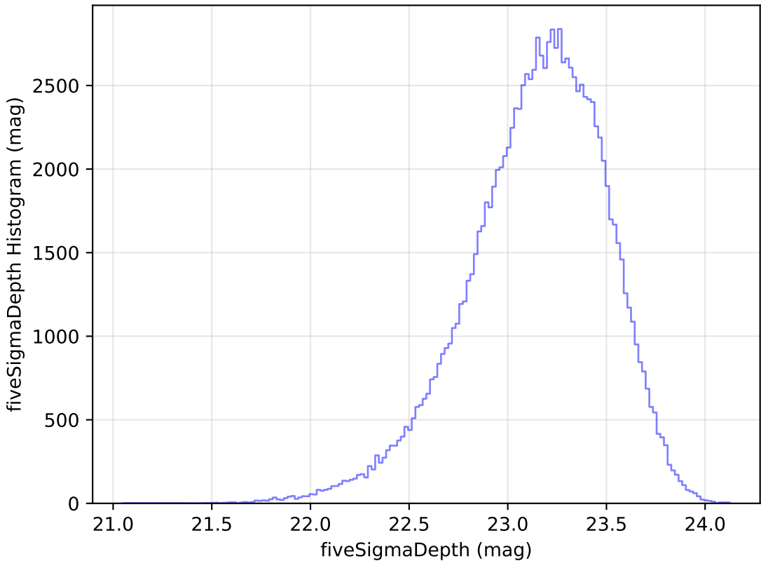
too_elab_r16_d3_giz_v3.4_10yrs u: fiveSigmaDepth Histogram
