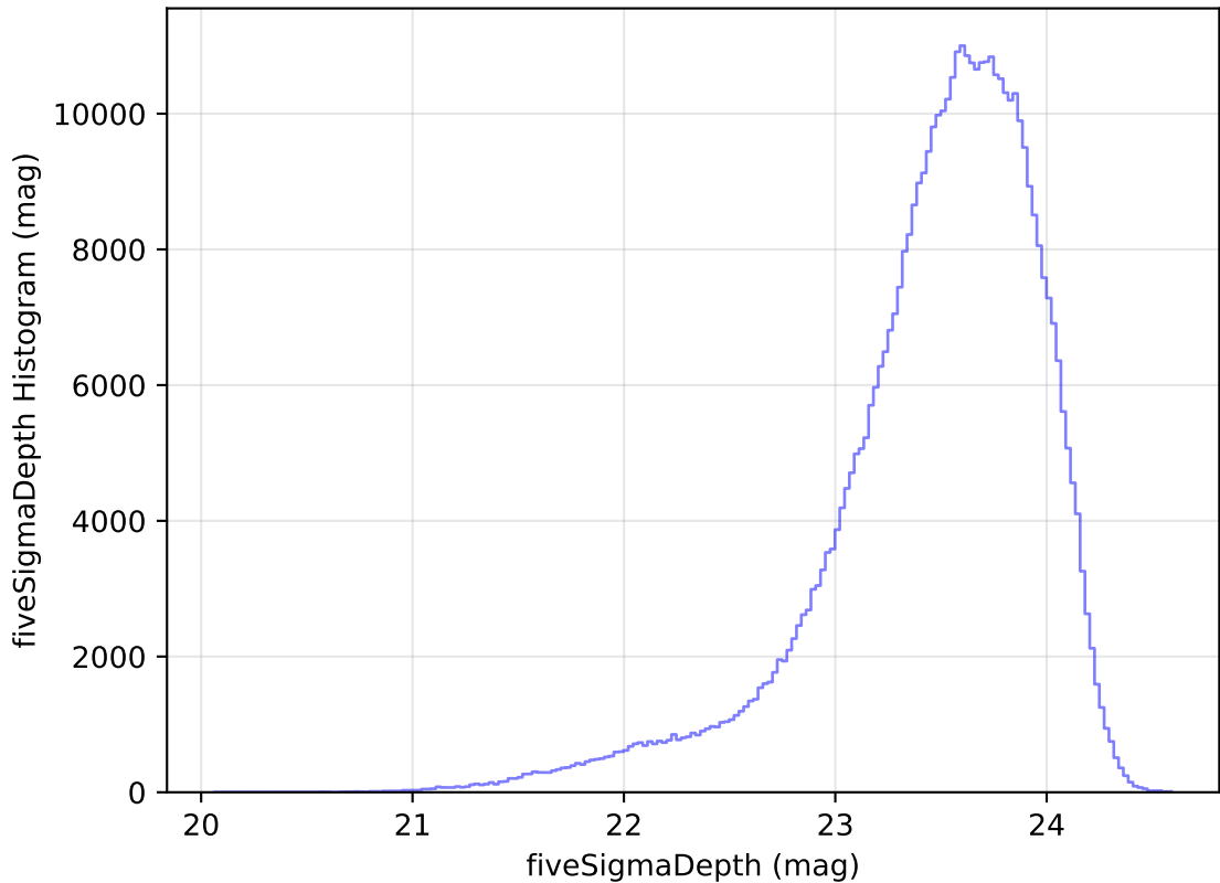
too_elab_r16_d3_giz_v3.4_10yrs i: fiveSigmaDepth Histogram
