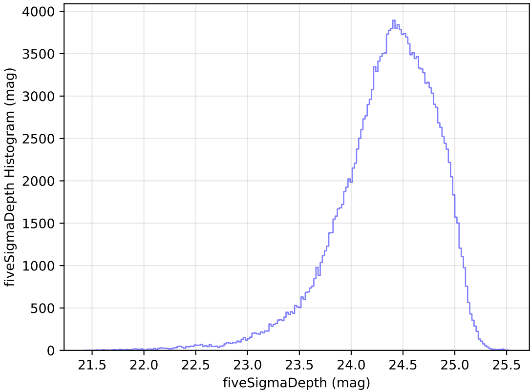
too_elab_r16_d3_giz_v3.4_10yrs g: fiveSigmaDepth Histogram
