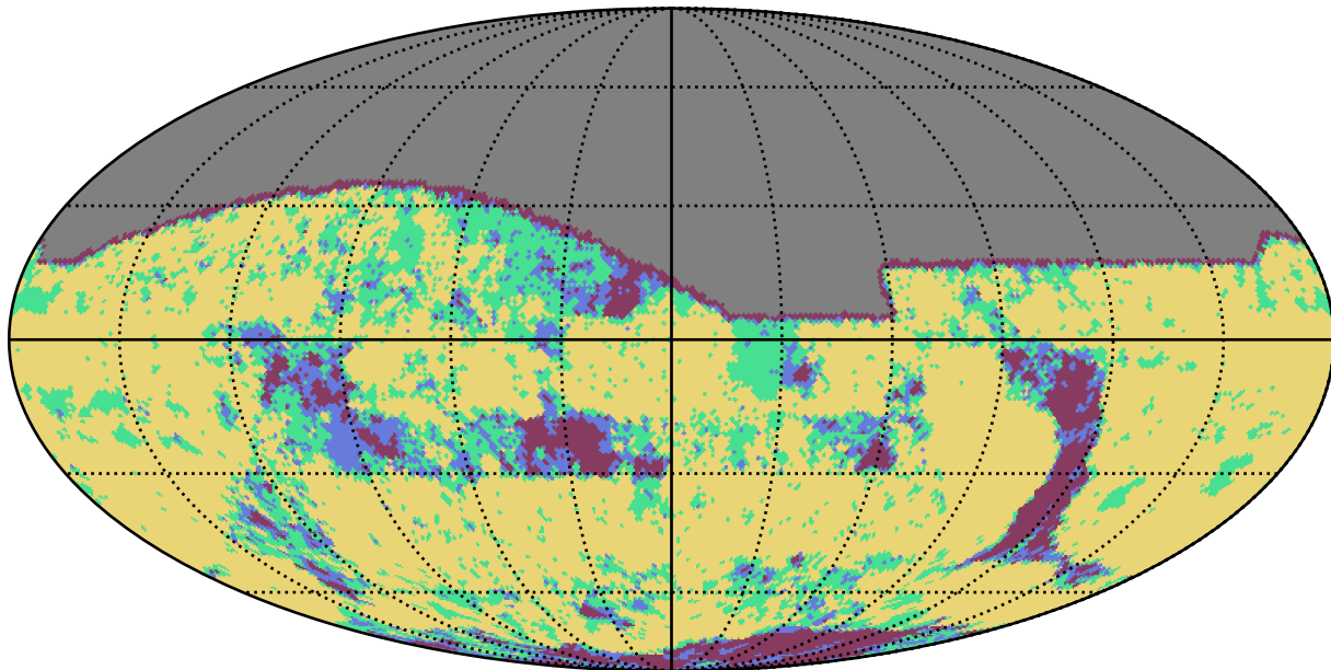
too_elab_r16_d3_giz_v3.4_10yrs g band: YearCoverage night
