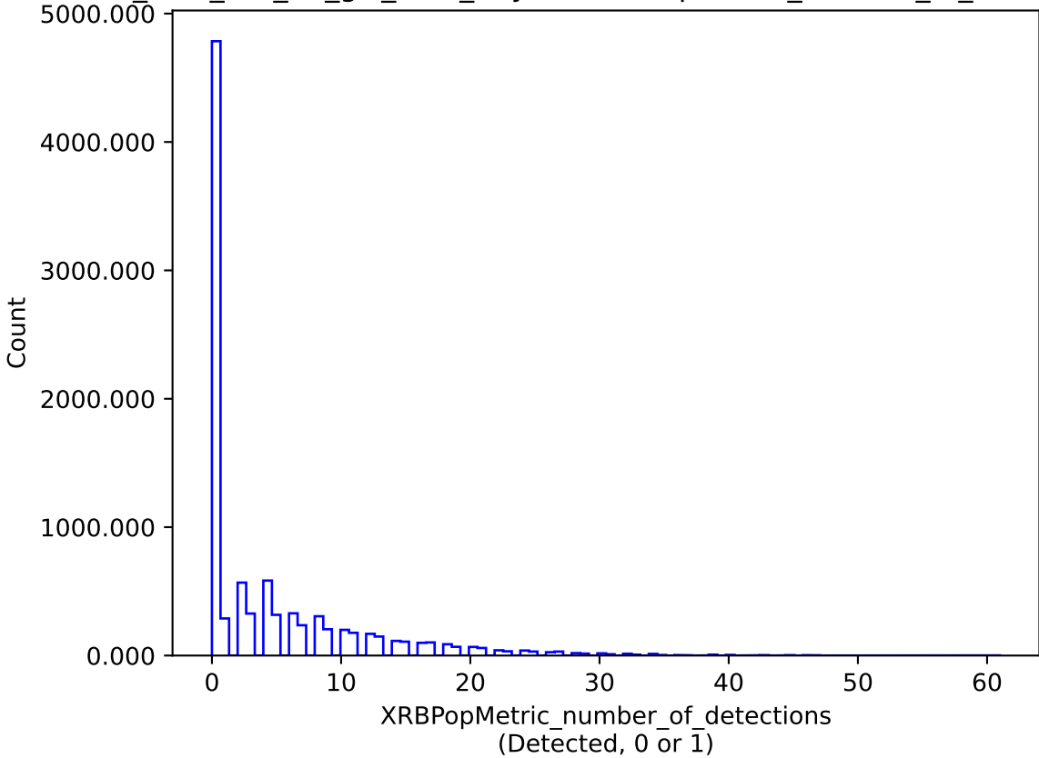
too_elab_r16_d3_giz_v3.4_10yrs : XRBPoMetric_number_of_detections
