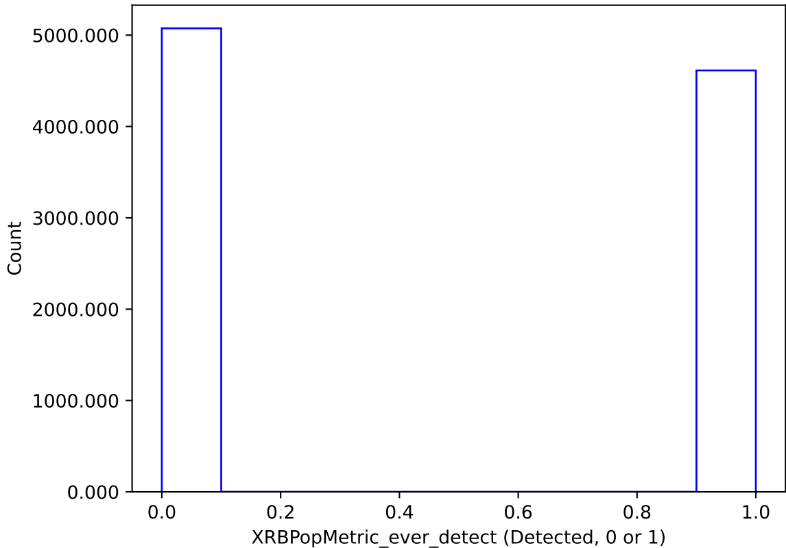
too_elab_r16_d3_giz_v3.4_10yrs : XRBPoMetric_ever_detect
