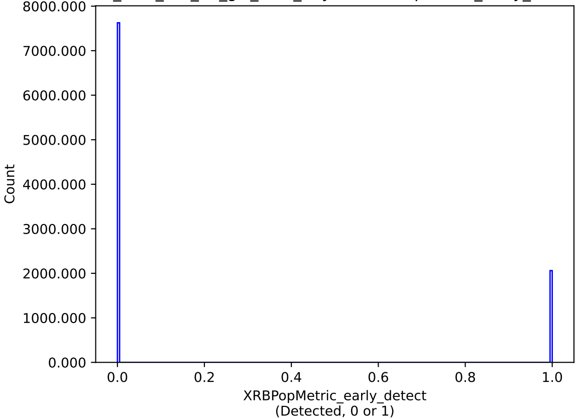
too_elab_r16_d3_giz_v3.4_10yrs : XRBPoMetric_early_detect
