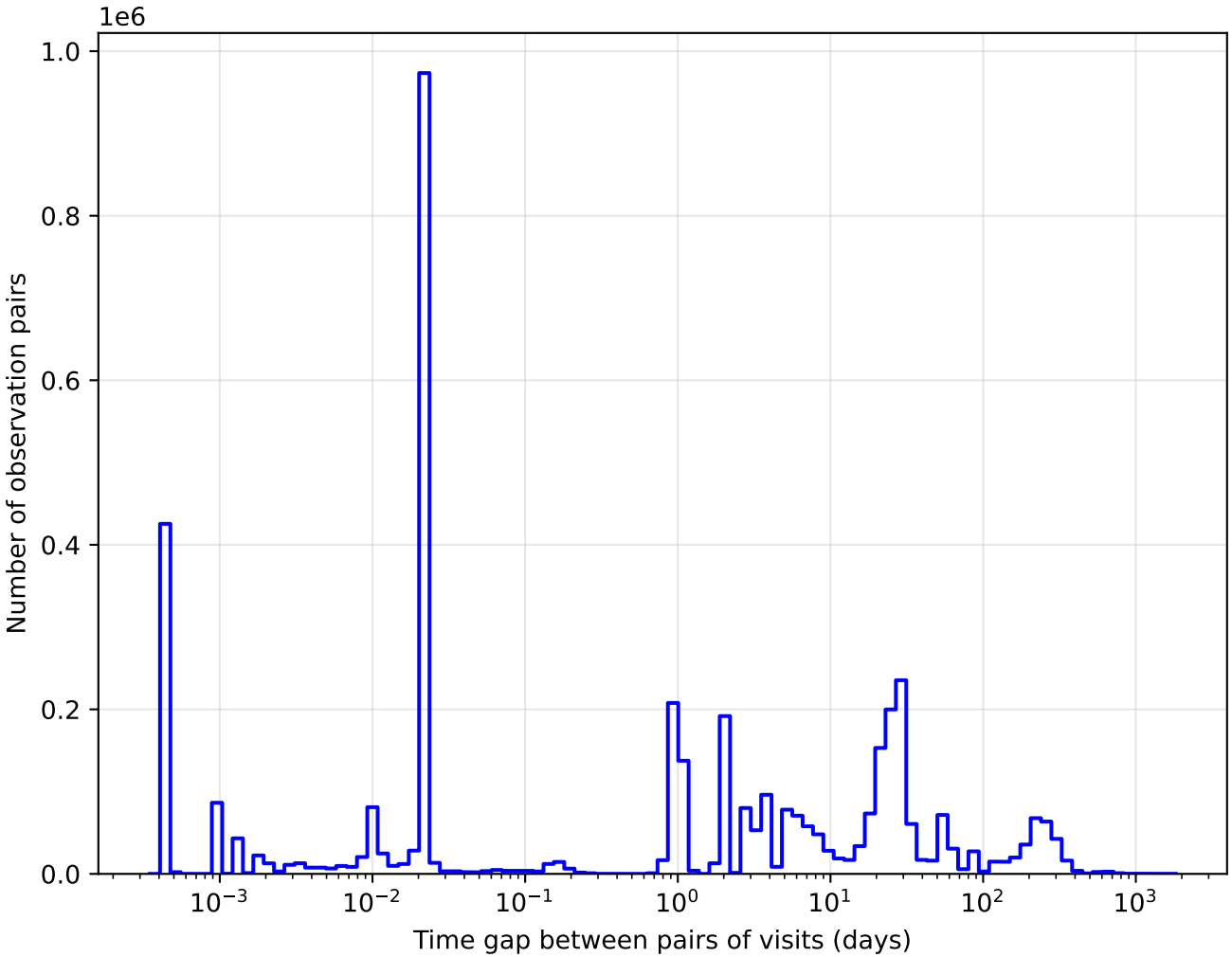
too_elab_r16_d3_giz_v3.4_10yrs y band: Tgaps observationStartMJD
