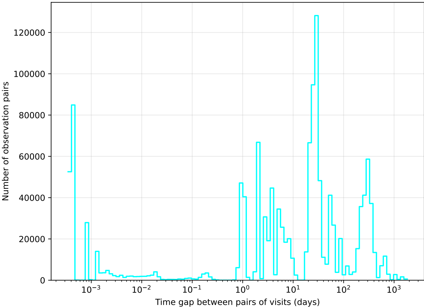
too_elab_r16_d3_giz_v3.4_10yrs u band: Tgaps observationStartMJD
