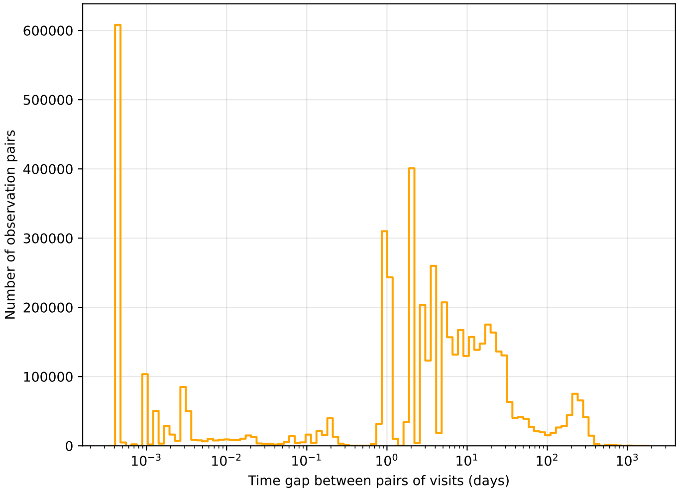
too_elab_r16_d3_giz_v3.4_10yrs r band: Tgaps observationStartMJD
