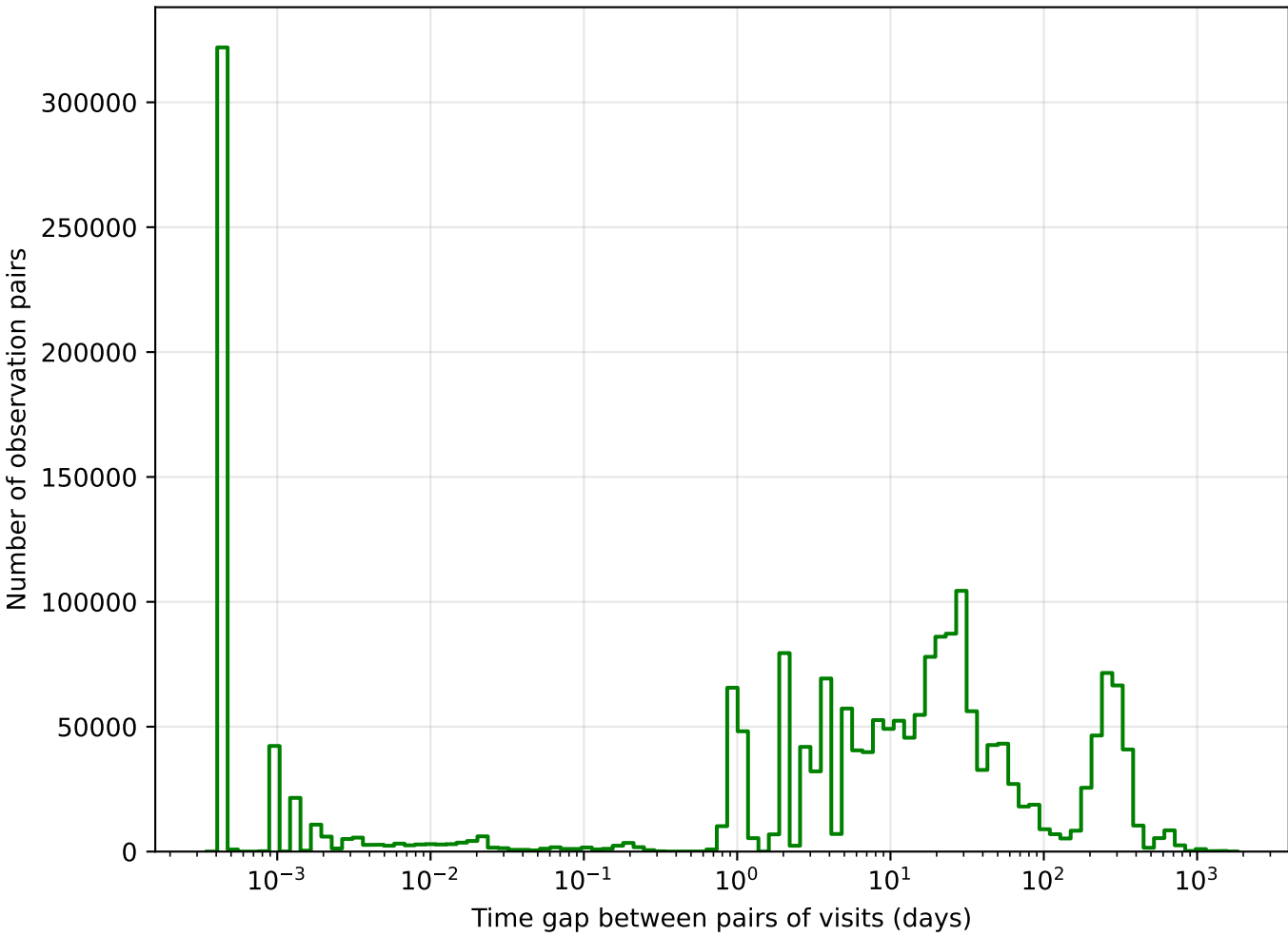
too_elab_r16_d3_giz_v3.4_10yrs g band: Tgaps observationStartMJD
