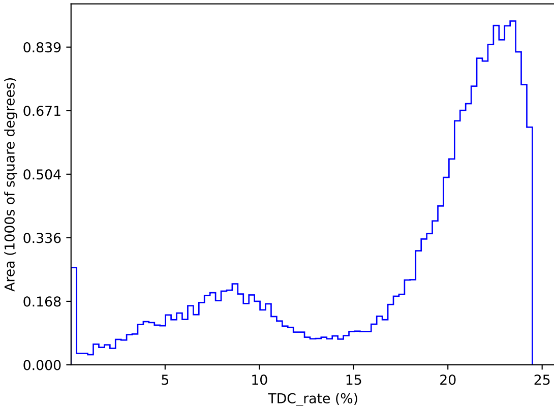
too_elab_r16_d3_giz_v3.4_10yrs : TDC_rate
