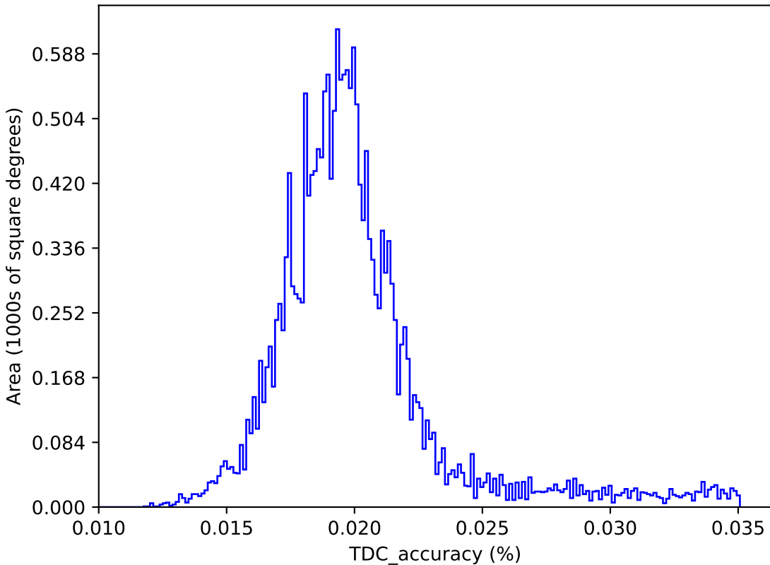
too_elab_r16_d3_giz_v3.4_10yrs : TDC_accuracy
