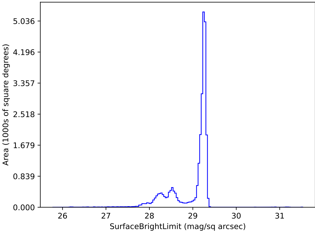
too_elab_r16_d3_giz_v3.4_10yrs z: SurfaceBrightLimit
