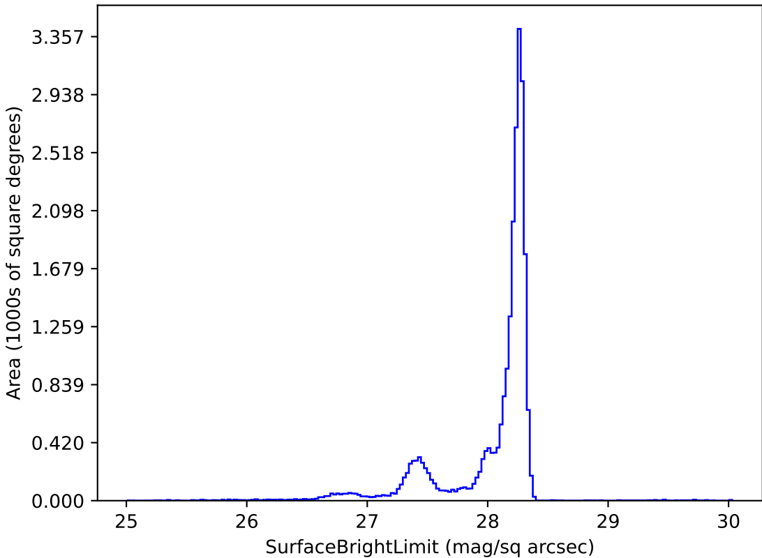
too_elab_r16_d3_giz_v3.4_10yrs y: SurfaceBrightLimit
