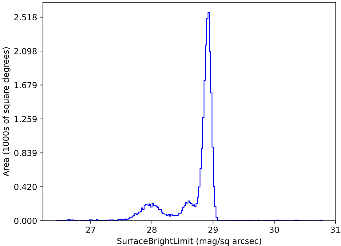
too_elab_r16_d3_giz_v3.4_10yrs u: SurfaceBrightLimit
