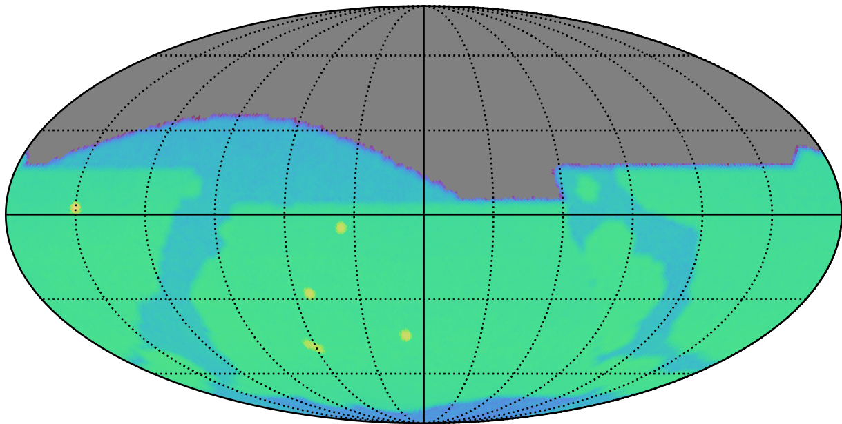
too_elab_r16_d3_giz_v3.4_10yrs r: SurfaceBrightLimit
