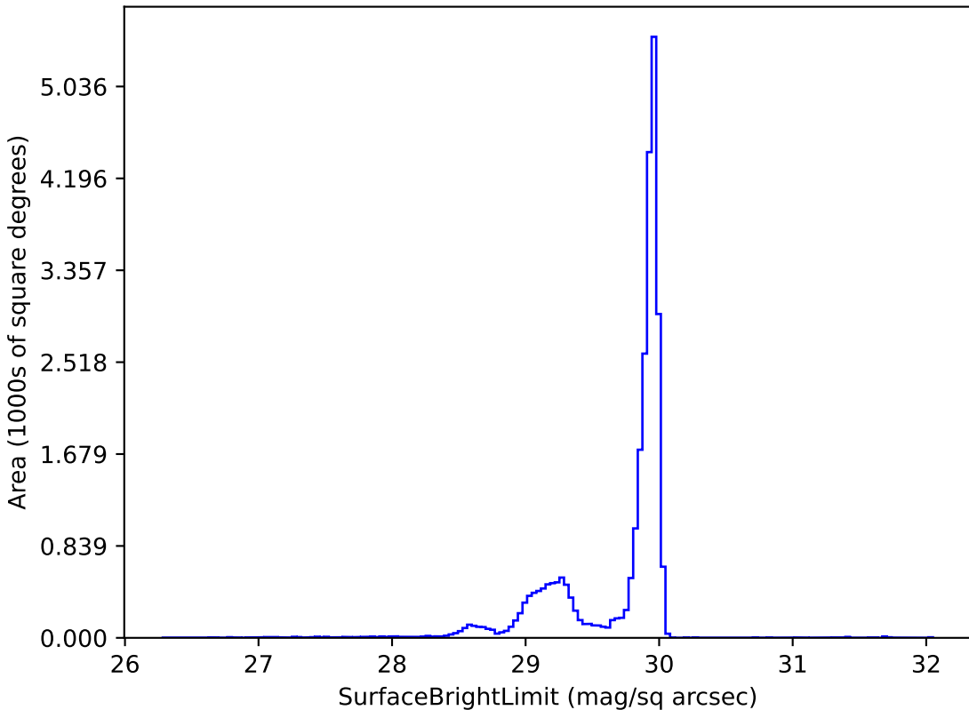
too_elab_r16_d3_giz_v3.4_10yrs i: SurfaceBrightLimit
