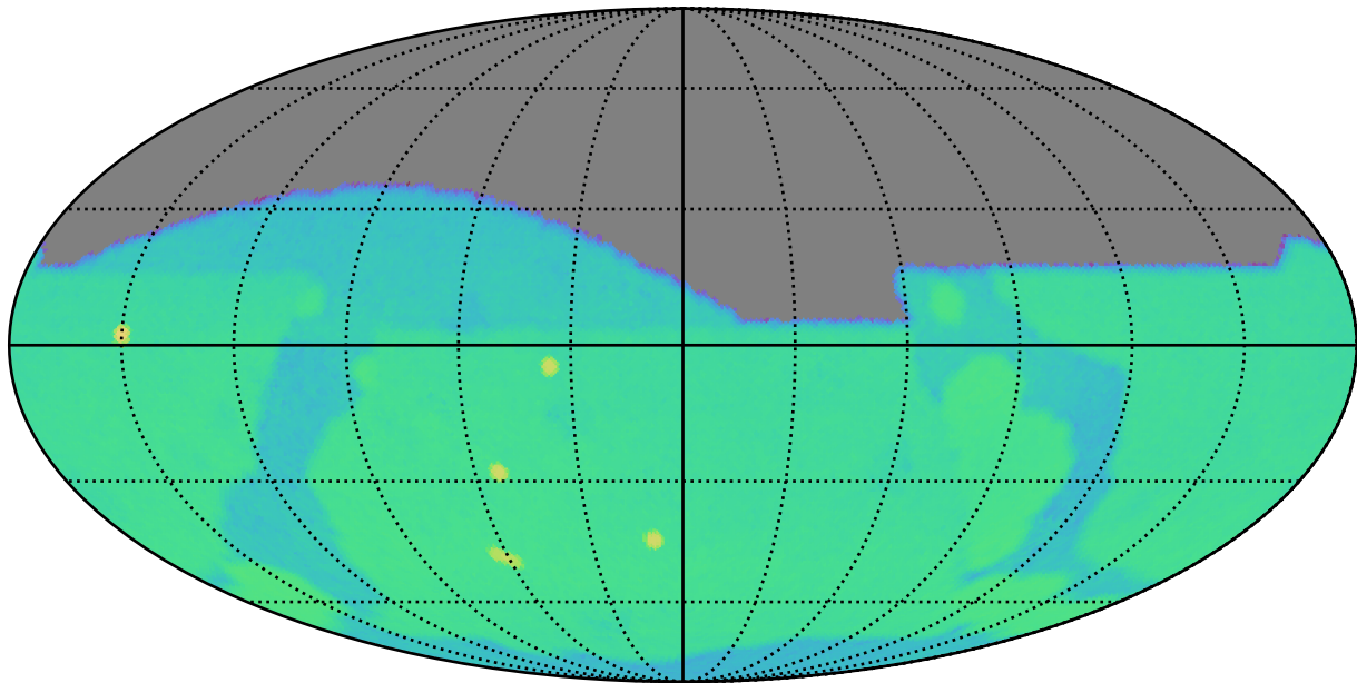
too_elab_r16_d3_giz_v3.4_10yrs g: SurfaceBrightLimit
