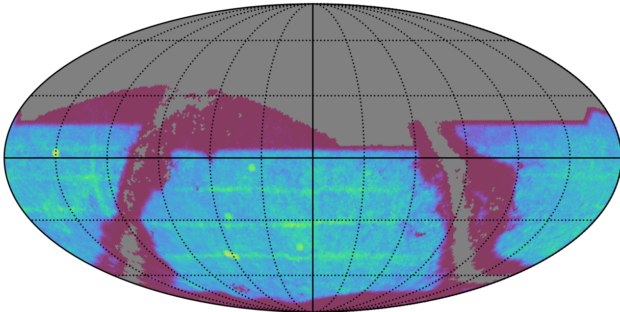
too_elab_r16_d3_giz_v3.4_10yrs : SNSLMetric
