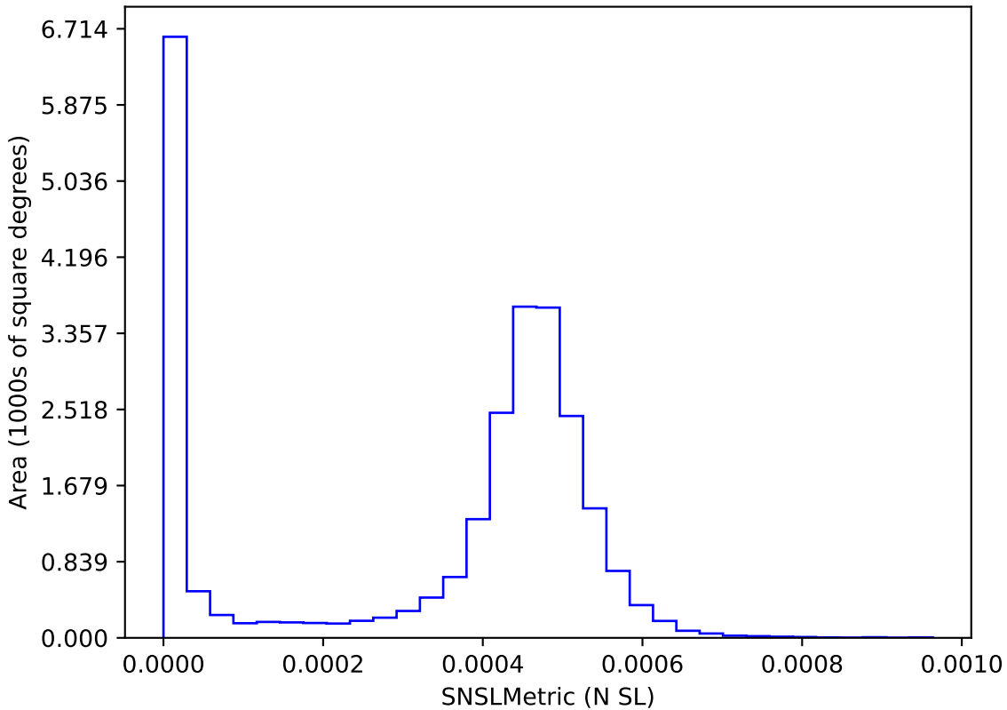
too_elab_r16_d3_giz_v3.4_10yrs : SNSLMetric
