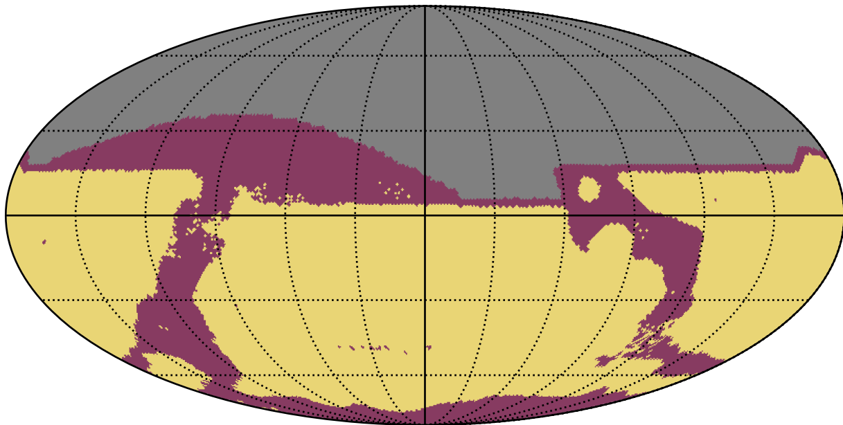
too_elab_r16_d3_giz_v3.4_10yrs : RapidRevisits
