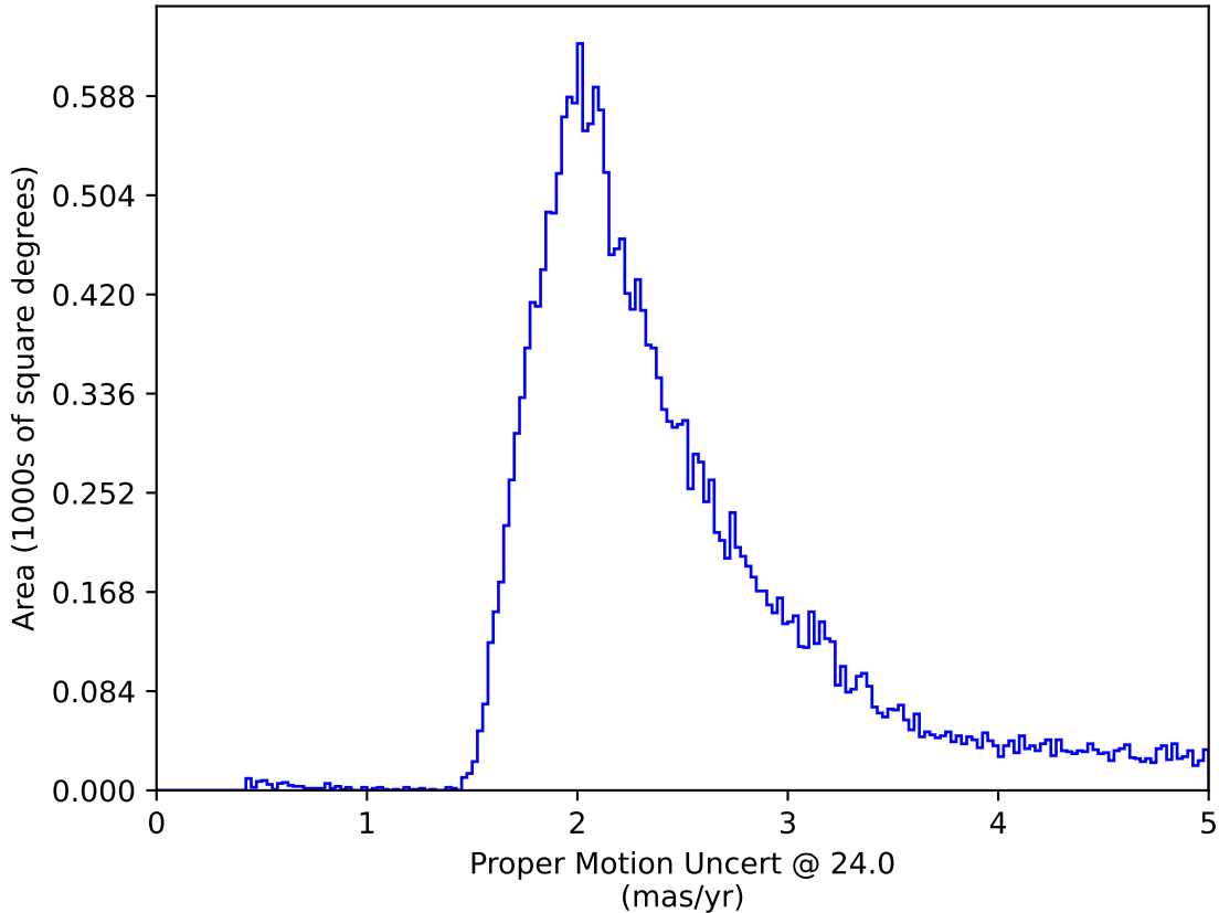
too_elab_r16_d3_giz_v3.4_10yrs : Proper Motion Uncert @ 24.0
