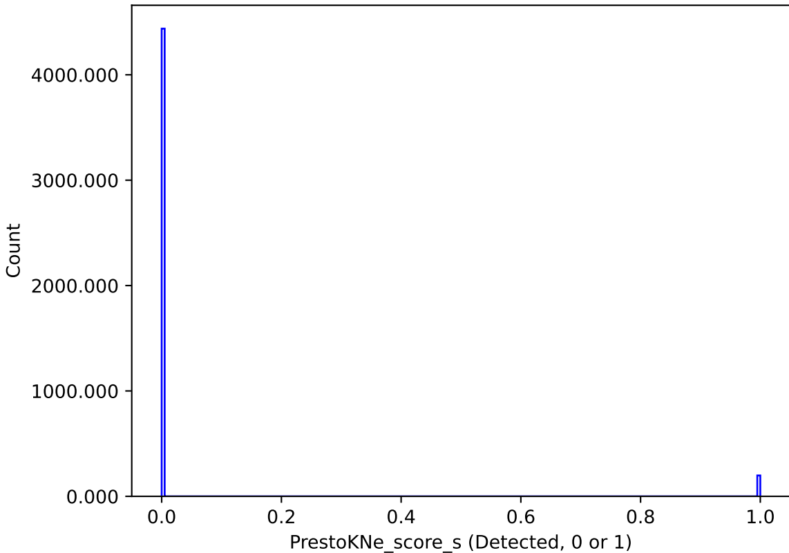
too_elab_r16_d3_giz_v3.4_10yrs : PrestoKNe_score_s
