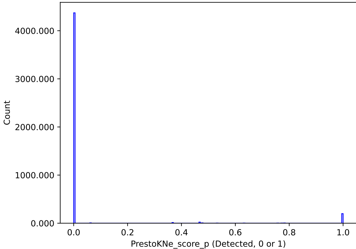
too_elab_r16_d3_giz_v3.4_10yrs : PrestoKNe_score_p
