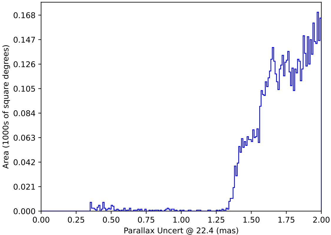
too_elab_r16_d3_giz_v3.4_10yrs : Parallax Uncert @ 22.4
