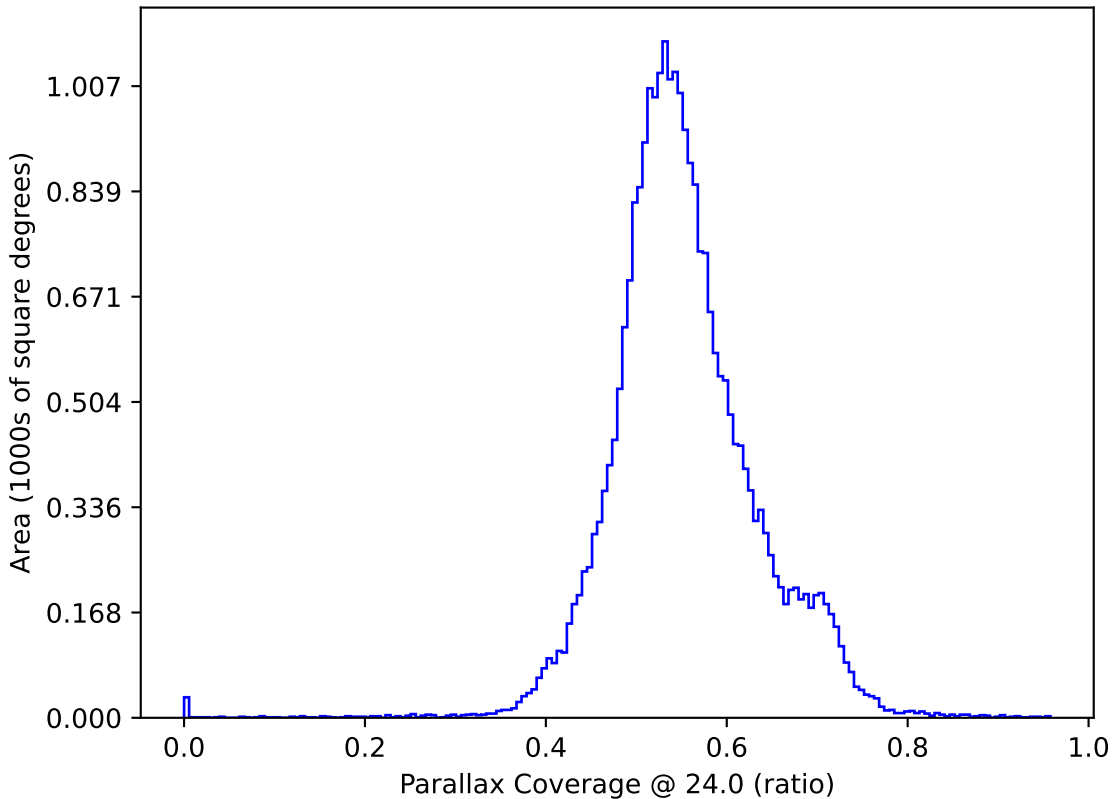
too_elab_r16_d3_giz_v3.4_10yrs : Parallax Coverage @ 24.0
