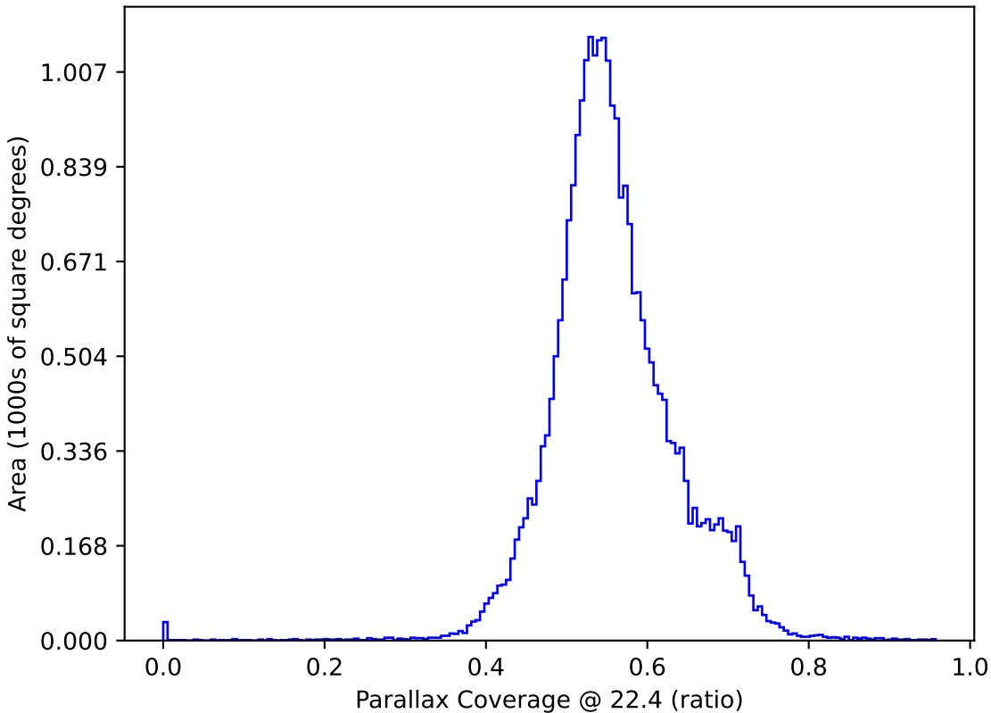
too_elab_r16_d3_giz_v3.4_10yrs : Parallax Coverage @ 22.4
