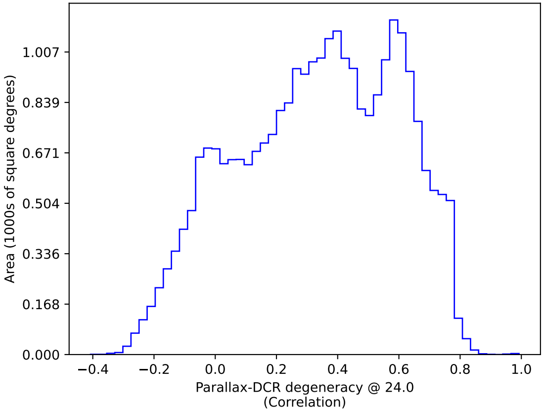
too_elab_r16_d3_giz_v3.4_10yrs : Parallax-DCR degeneracy @ 24.0
