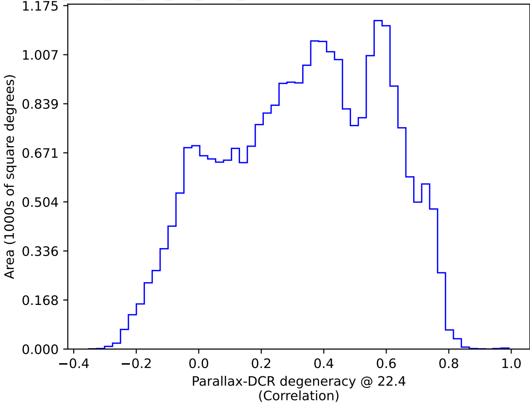
too_elab_r16_d3_giz_v3.4_10yrs : Parallax-DCR degeneracy @ 22.4
