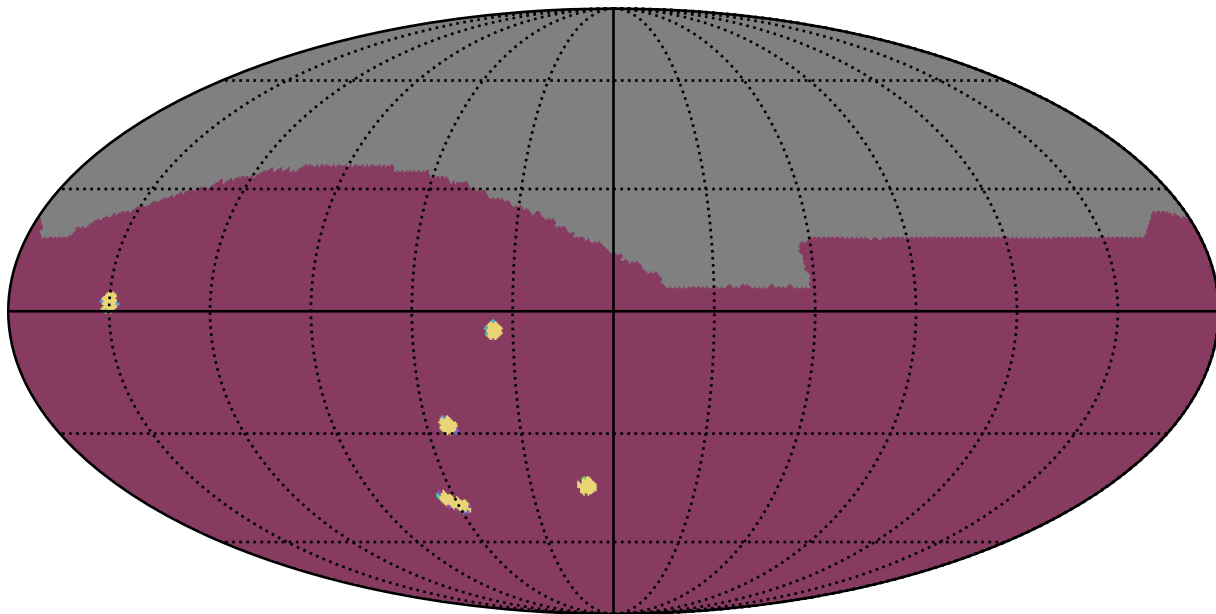
too_elab_r16_d3_giz_v3.4_10yrs : NumberOfQuickRevisits
