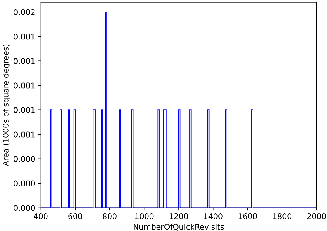
too_elab_r16_d3_giz_v3.4_10yrs : NumberOfQuickRevisits
