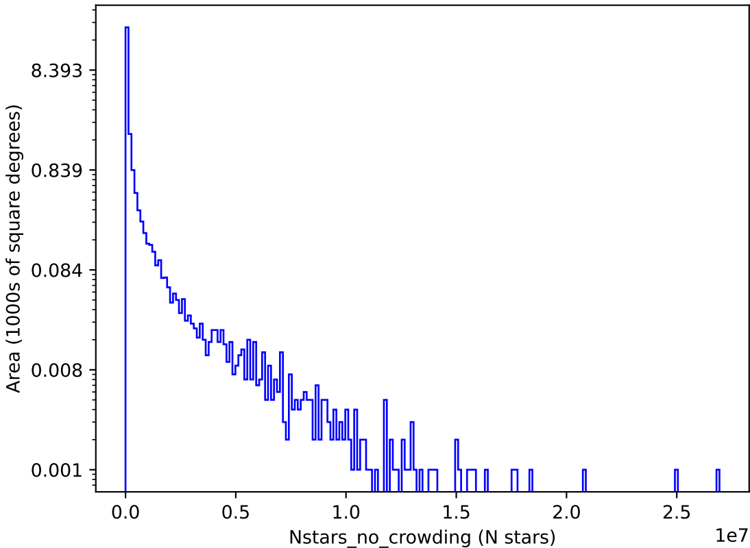
too_elab_r16_d3_giz_v3.4_10yrs i: Nstars_no_crowding
