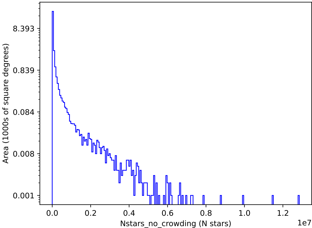
too_elab_r16_d3_giz_v3.4_10yrs g: Nstars_no_crowding
