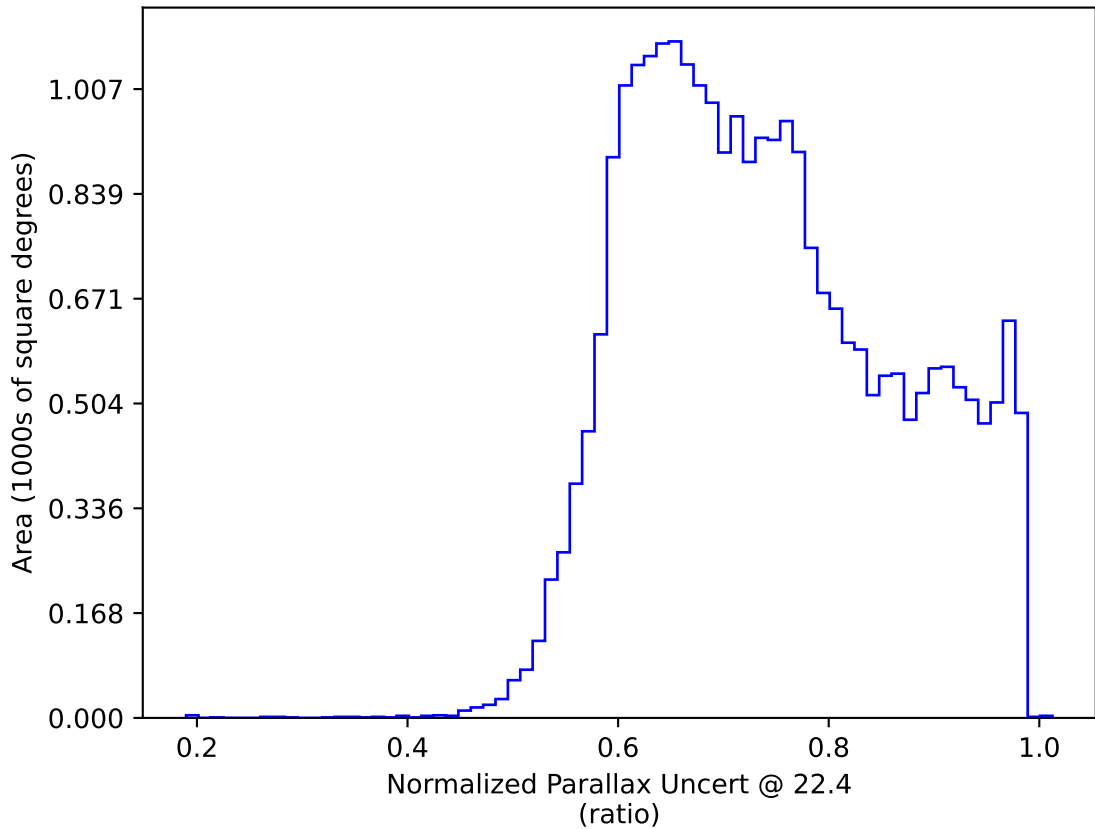
too_elab_r16_d3_giz_v3.4_10yrs : Normalized Parallax Uncert @ 22.4
