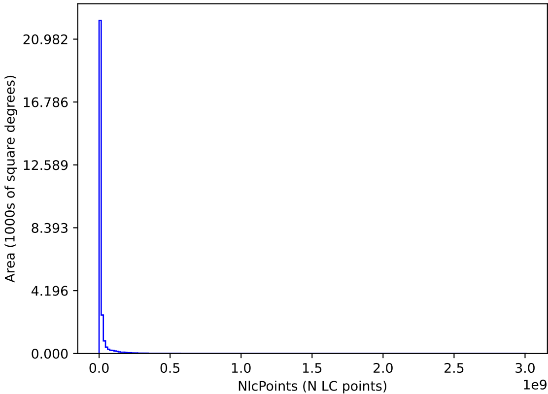
too_elab_r16_d3_giz_v3.4_10yrs : NlcPoints
