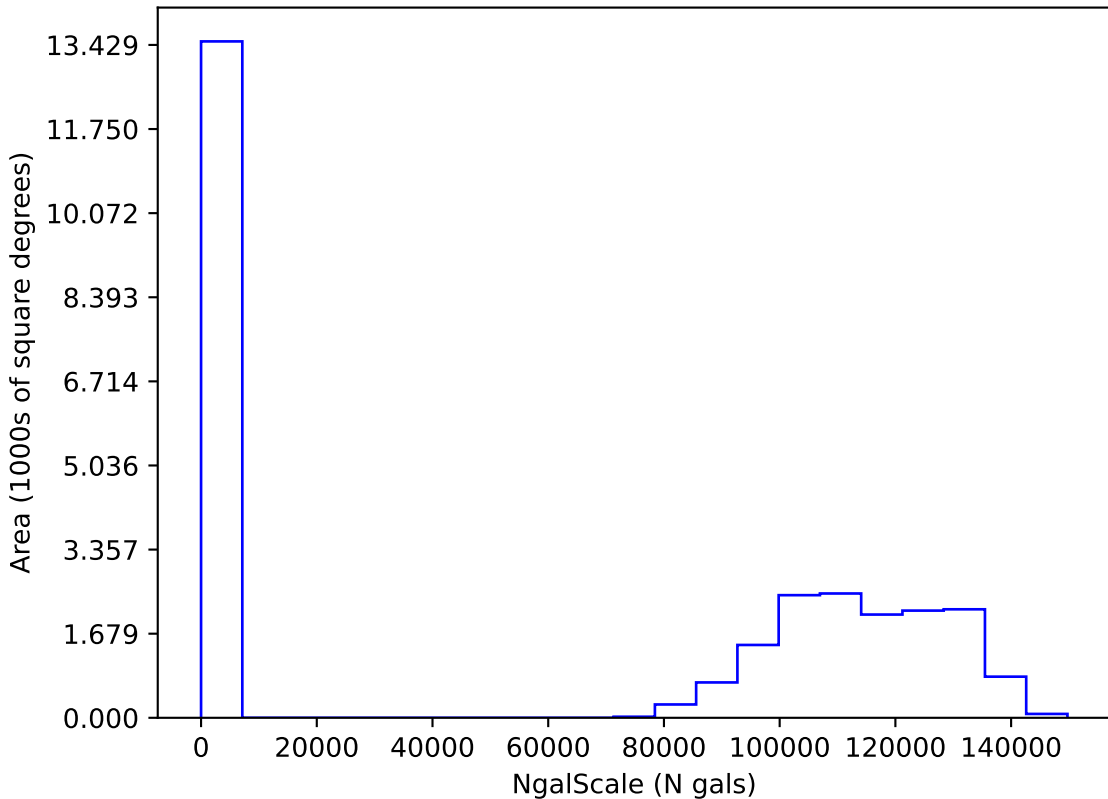
too_elab_r16_d3_giz_v3.4_10yrs i: NgalScale
