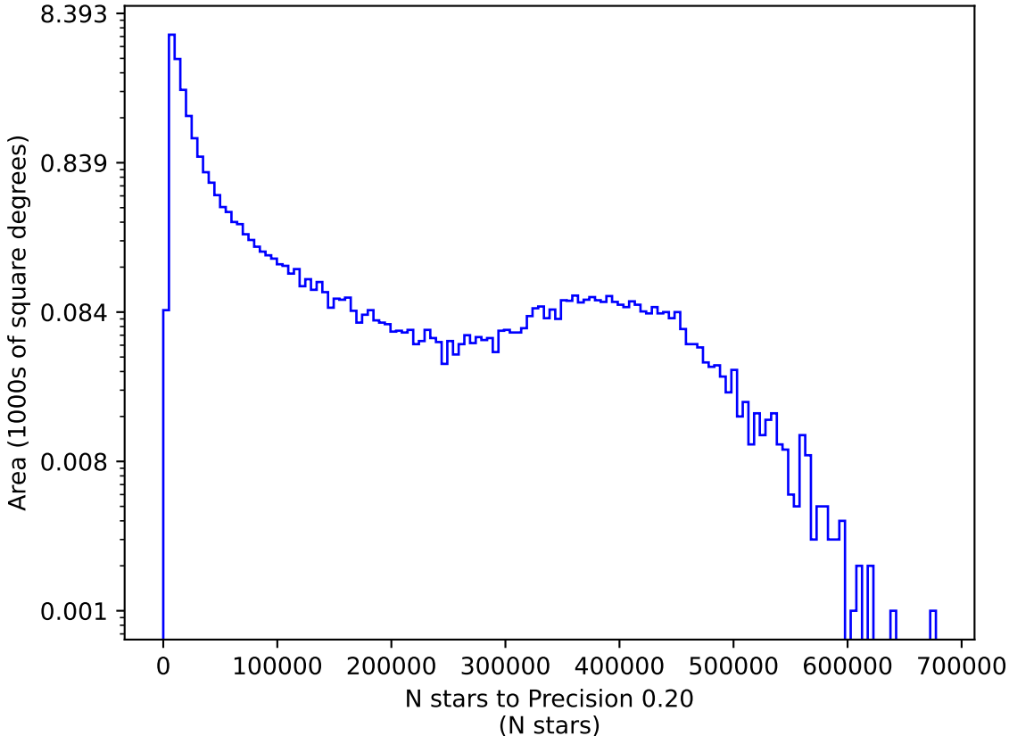
too_elab_r16_d3_giz_v3.4_10yrs z: N stars to Precision 0.20
