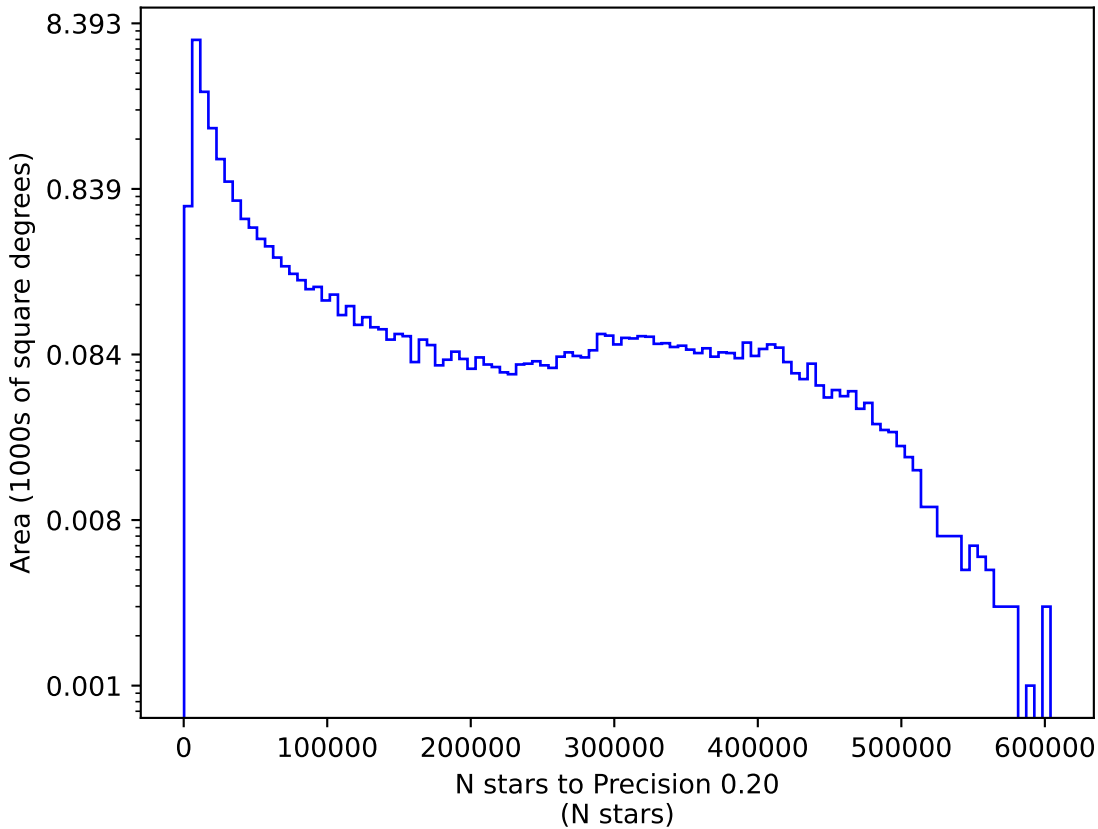
too_elab_r16_d3_giz_v3.4_10yrs y: N stars to Precision 0.20
